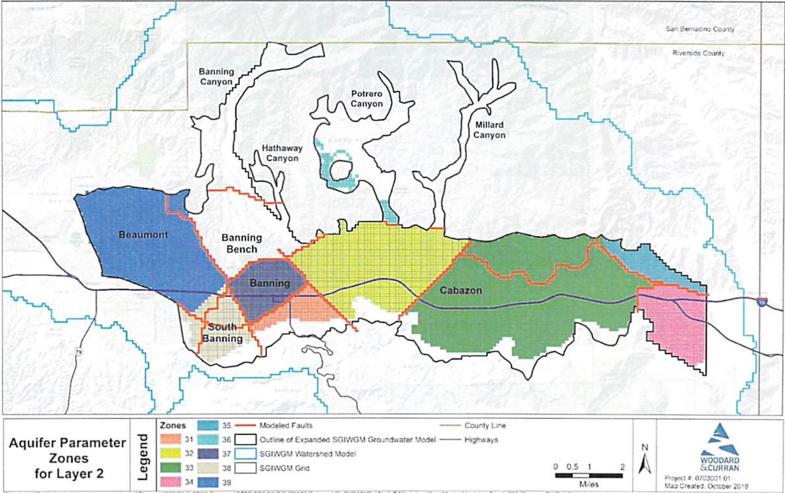
Figure 13: Layer 2 Aquifer Zones
