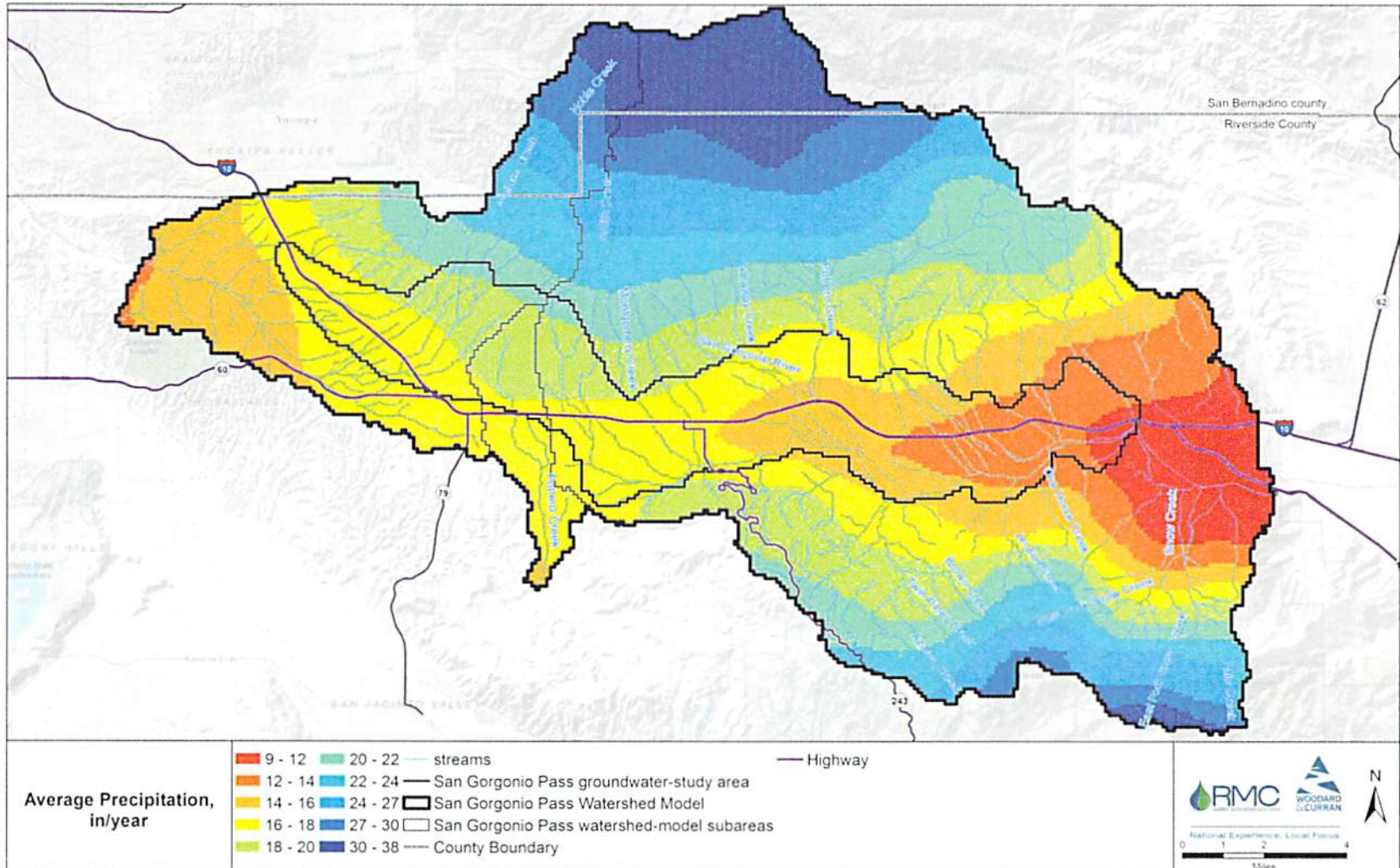
Figure 19 – PRMS Average Precipitation (30 years, 1983-2012) (Note: Groundwater study area refers to USGS model)
