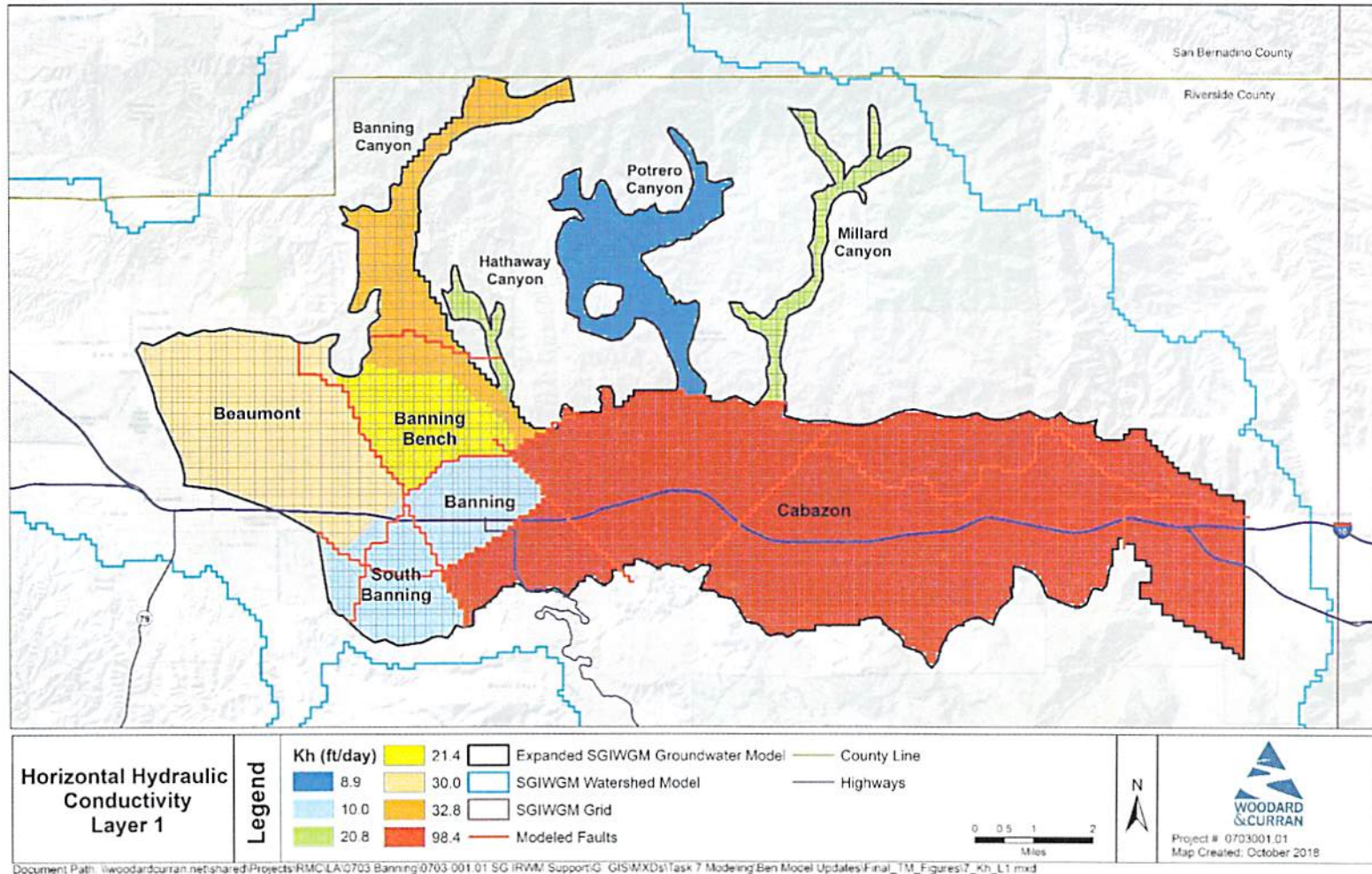
Figure 16: Layer 1 Horizontal Hydraulic Conductivity
