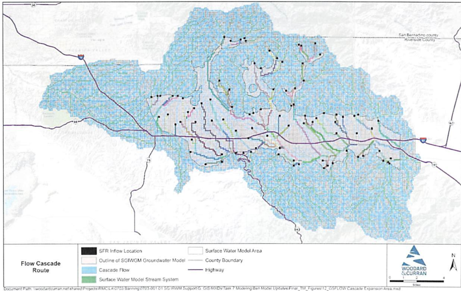
Figure 22: Flow Cascade Route
