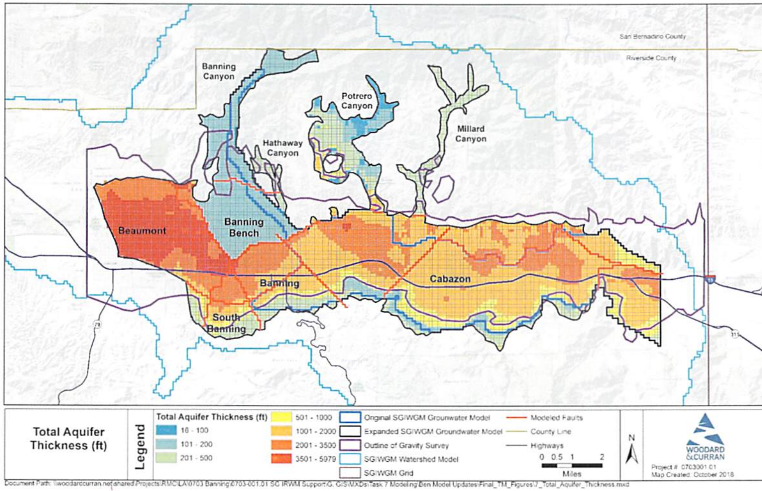
Figure 7: Total Aquifer Thickness for SGIWGM Groundwater Model
