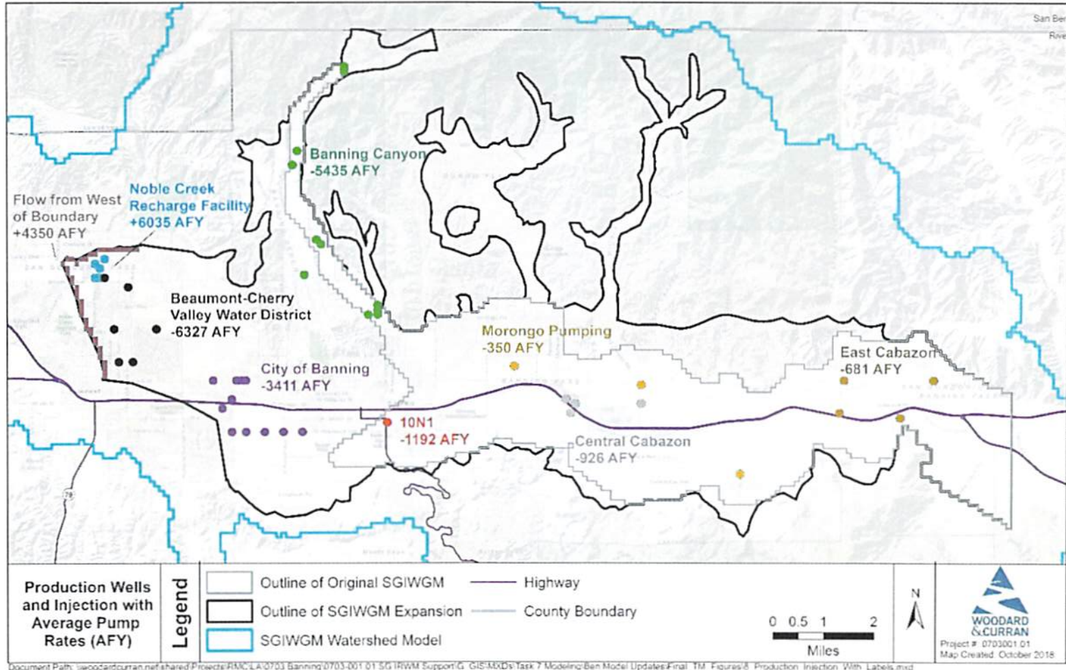
Figure 18: Average Production and Injection Rates (AFY) for Simulation Period
