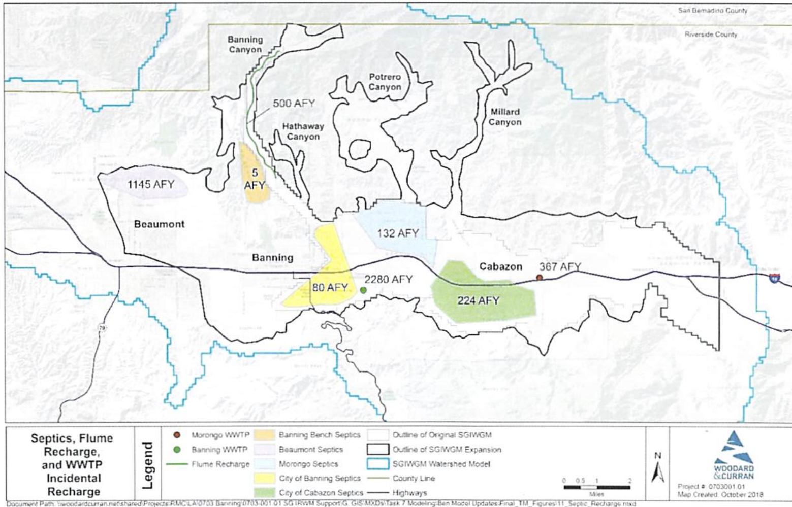
Figure 21: Septic and WWTP Recharge
