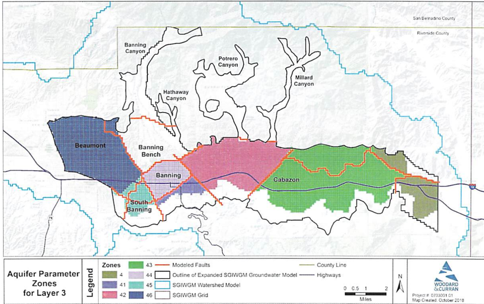
Figure 14: Layer 3 Aquifer Zones
