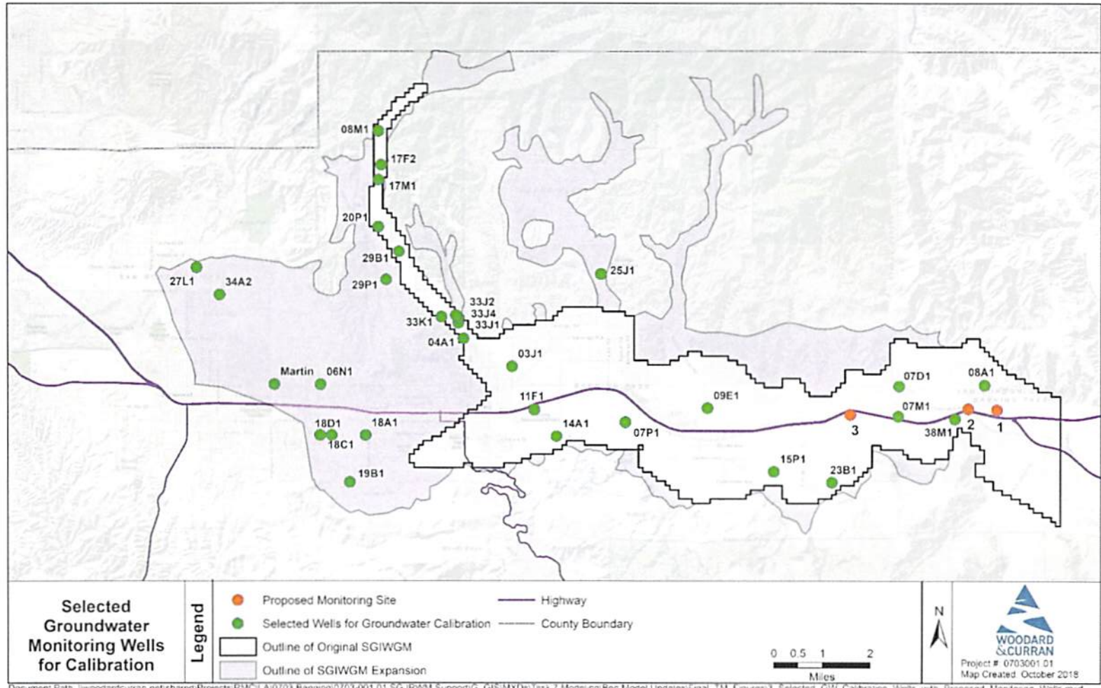
Figure 25: Monitoring Wells Selected for Calibration of Expanded SGIWGM
