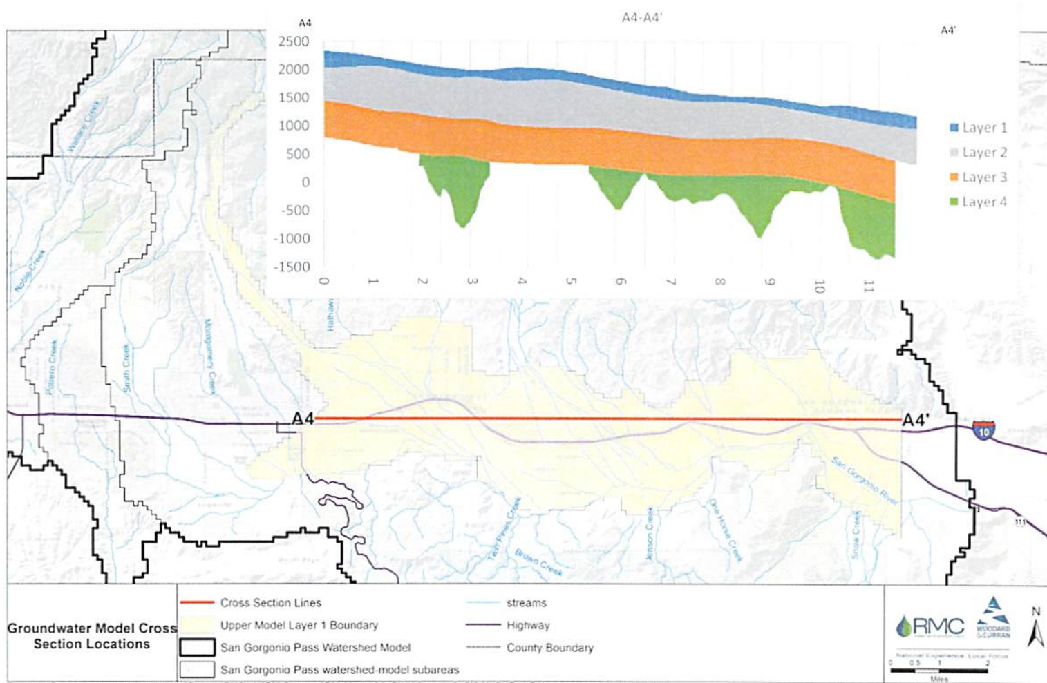
Figure 32 – SGIWGM Cross Section A4-A4'
