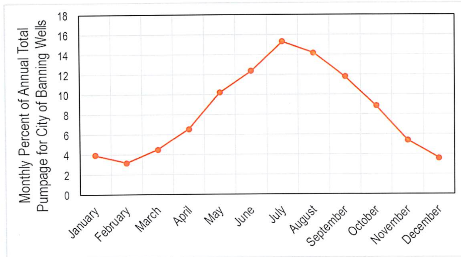
Figure 19: Monthly Pumpage Percentage
