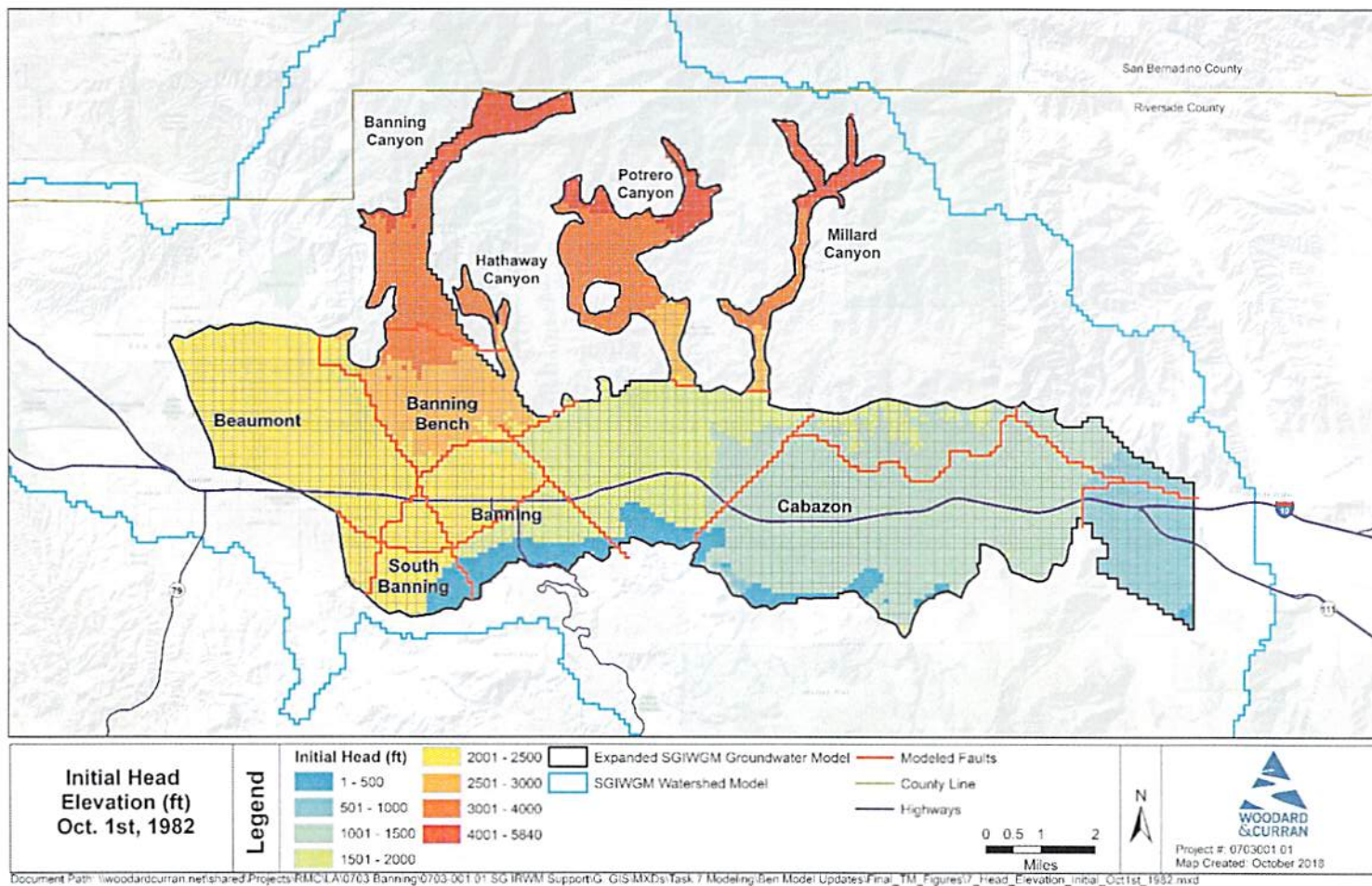
Figure 17: Initial Heads (October 1st, 1982)
