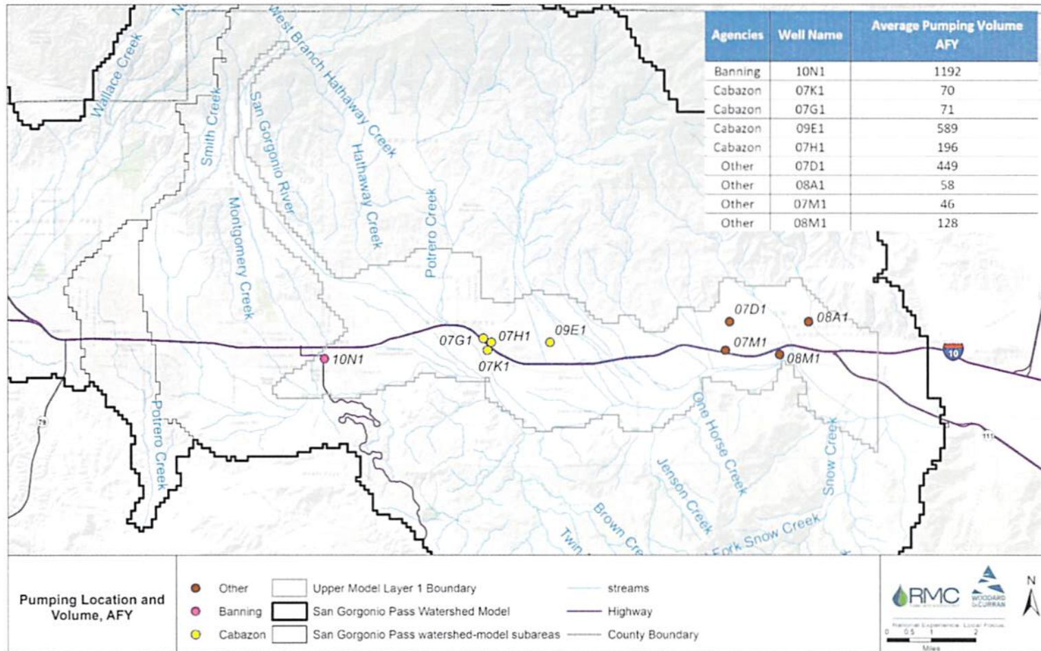
Figure 13 – Location of Wells and Average Pumping Rates for 2010-2012 period in LM
