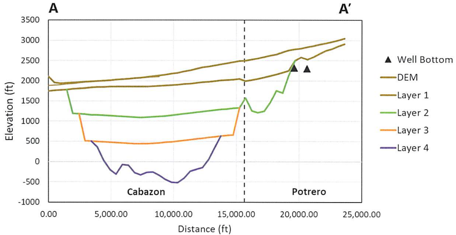
Figure 9: Cross-Section A-A' (Cabazon to Potrero Canyon, S-N)
