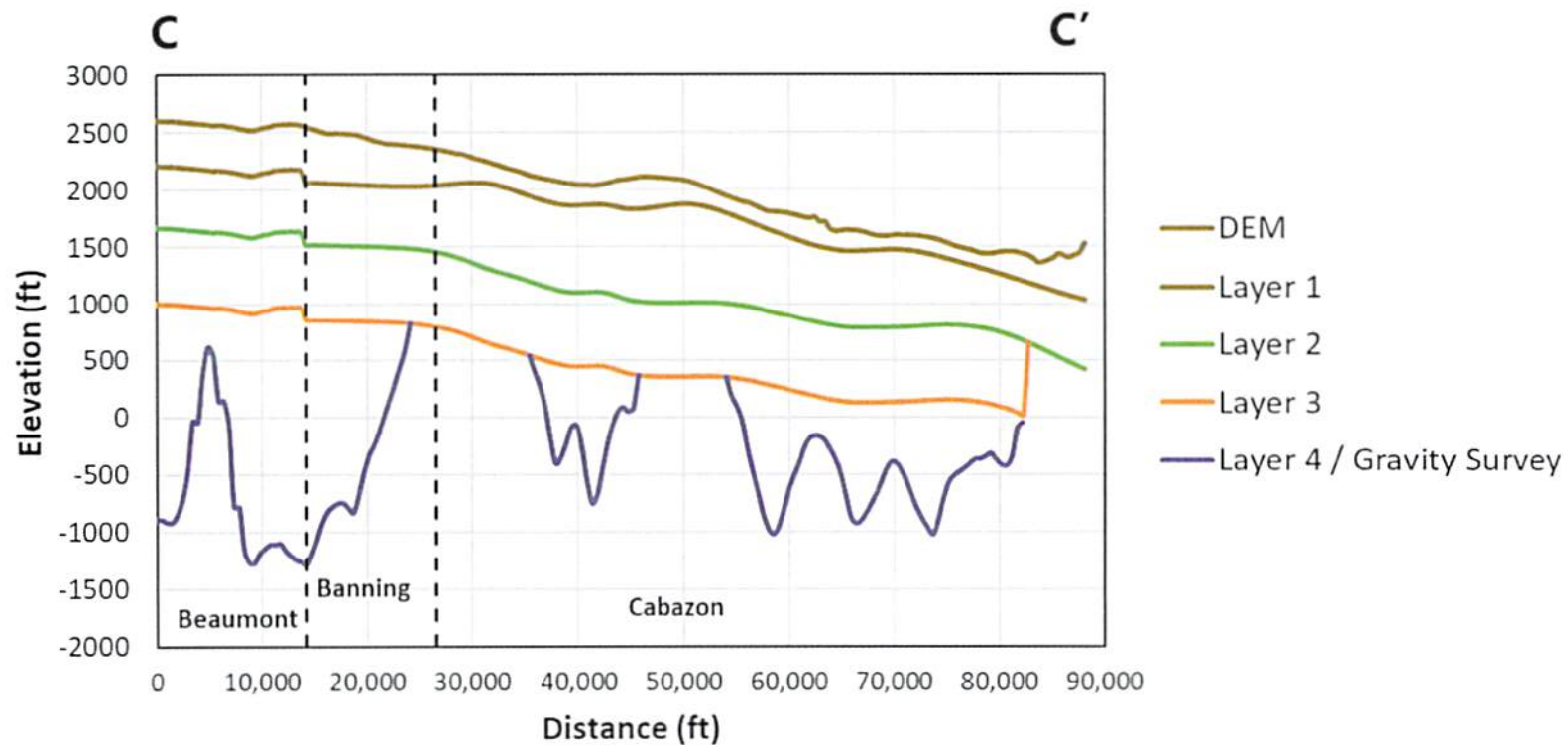
Figure 11: Cross-Section C-C' (Beaumont to Cabazon, W-E)
